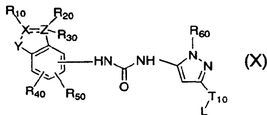
Formula (X)
